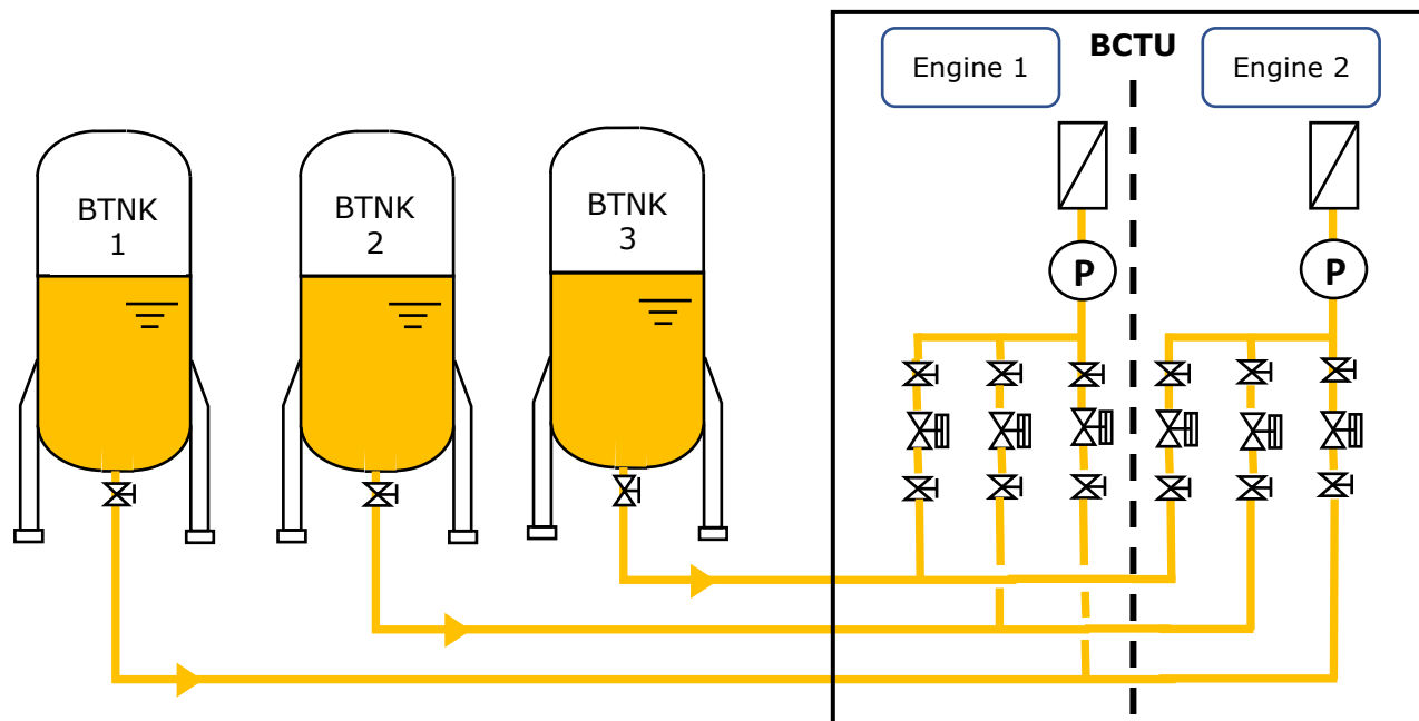
Figure 5 – Configuration of Multiple Bulk Tank connection to BCTU Pumps
