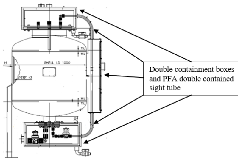
Figure 6 – Typical Tank drawing with containment boxes
