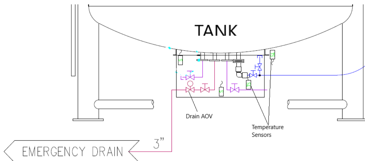
Figure 9 – Proposed location of Temperature Sensors and Drain AOV at tank bottom
