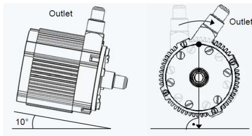
Figure 4 - Forward incline (Left) / Turned Pump (Right)
