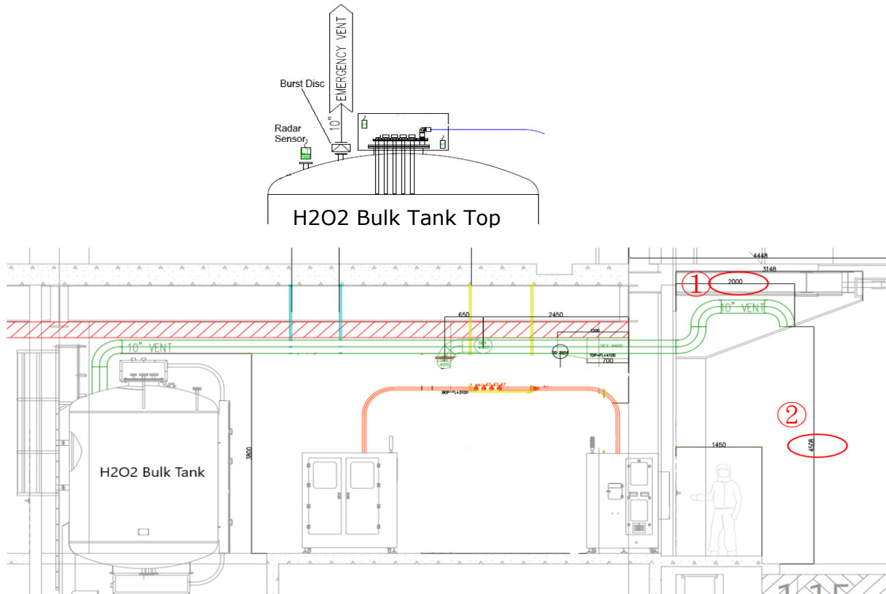
Figure 10 – Illustration of H 2 O 2 Bulk Tank Vent line Installation
